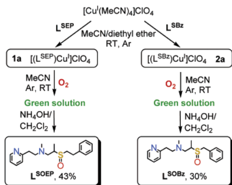
Figure 3. Synthesis of thioether ligand–copper(I) complexes and their reactivity toward O_2 , producing sulfoxide products.
