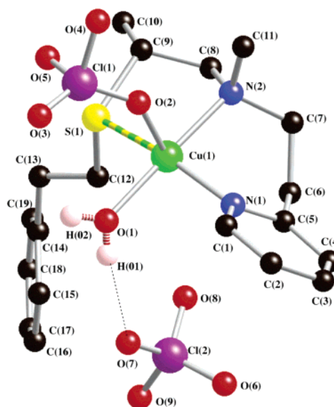
Figure 7. Crystal structure of [(L^{\text{SEP}})\text{Cu}^{\text{II}}(\text{H}_2\text{O})(\text{OCIO}_3)](\text{ClO}_4) ( 1b ). Hydrogen atoms are omitted for clarity.
