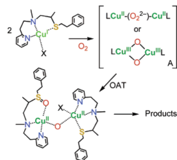
Figure 4. Possible course of reaction for ligand sulfoxidation by Cu^I/O_2 with L^{SEP} .
