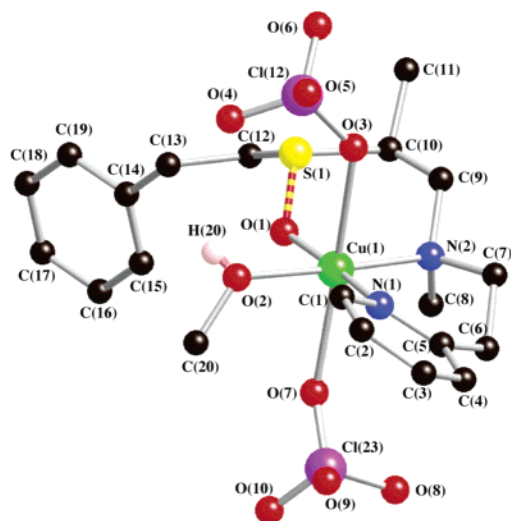
Figure 5. X-ray crystal structure of [(L^{\text{SOEP}})\text{Cu}^{\text{II}}(\text{CH}_3\text{OH})(\text{OCIO}_3)_2] . The hydrogen atoms have been omitted for clarity.
