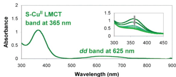
Figure 8. UV–vis spectra of [(L^{SEP})Cu^{II}(H_2O)(OCIO_3)]ClO_4 \cdot H_2O in MeCN. Inset: 365 nm band decrease while the temperature is increased from -40 °C to RT after addition of H_2O_2 .
